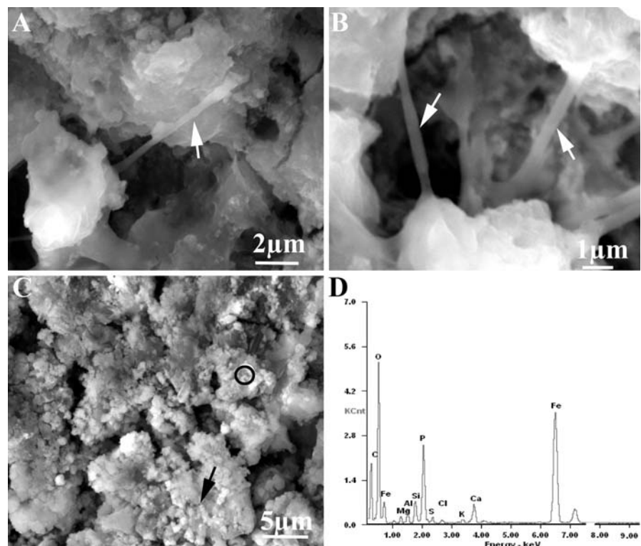
Fig. 2 a, b Environmental scanning electron microscope (ESEM) images of tubeworms show filamentous microorganisms (white arrows) occur in the interspace layer of the tube wall. c Numerous Fe oxides (black arrow) form on the outer tube wall surface. d The energy spectrum analysis of the outer tube wall surface (black cycle) in c . The contents of Fe, P, Ca and O are higher, indicating that Fe occurs as Fe oxides
