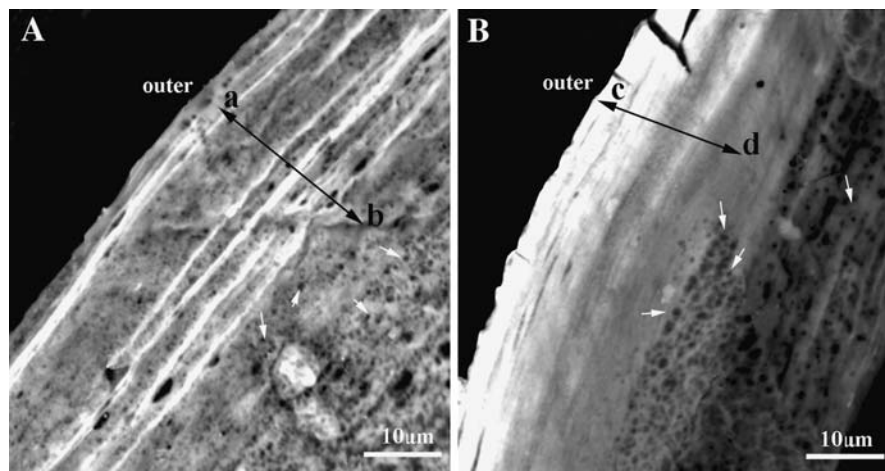
Fig. 5 BSE (back-scattered electron) images of tube walls. a Electron lucent areas within the tube wall are parallel to the tube wall surface and exhibit a laminated structure. b Electron lucent degree is generally enhanced from inside to outside across the tube wall. Black spots (white arrows) are inferred to
