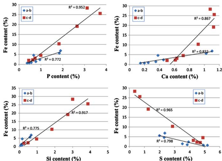
Fig. 6 Chemical element analysis of EPMA to line ab and cd in Fig. 5 shows Fe contents have a good positive correlation with Ca, P and Si, but have a negative correlation with S
