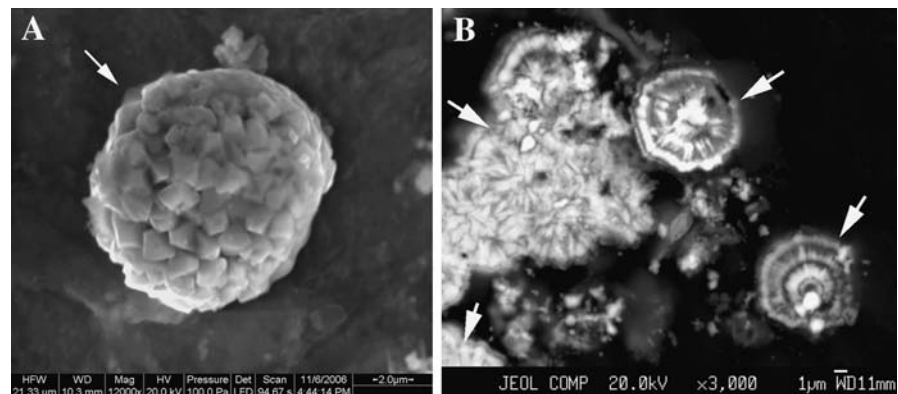
Fig. 4 Framboidal pyrites are observed on the surface of internal tube wall. a ESEM image. b BSE (back-scattered electron) image
