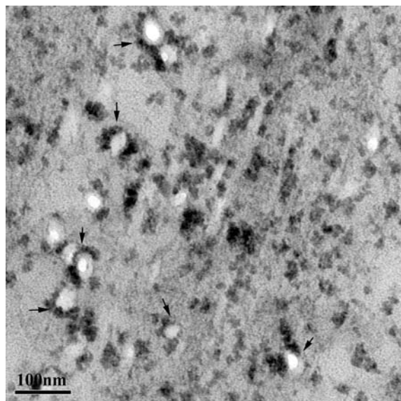
Fig. 8 TEM image shows degradation products of microorganisms distribute within the tube wall. Black arrows show that some cells totally degrade and degradation products envelope the residual holes
