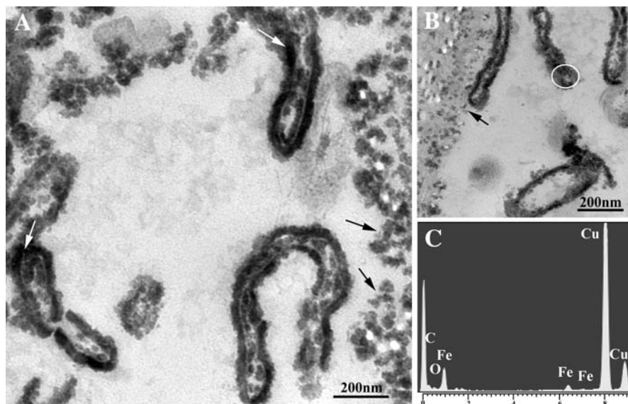
Fig. 7 TEM microphotographs with EDS reveal that the microorganisms in the tube wall are enveloped by Fe oxides. White arrows show the extracellular precipitates on the surface of cells. Black arrows point to nano particles possibly formed by the degradation of microorganisms. EDS analysis of extracellular precipitates (white circle) in band show higher Fe and O are detected. Cu peak comes from Cu net
